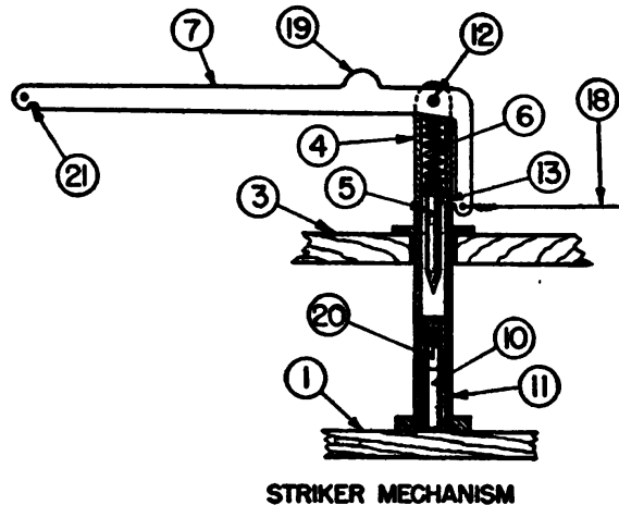
FIGURE 76.—Improvised mine, HE shells—detail.
